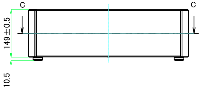
A view
