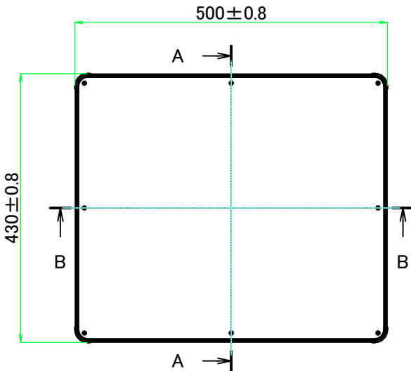
E view
