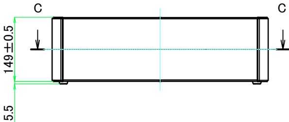
A view
