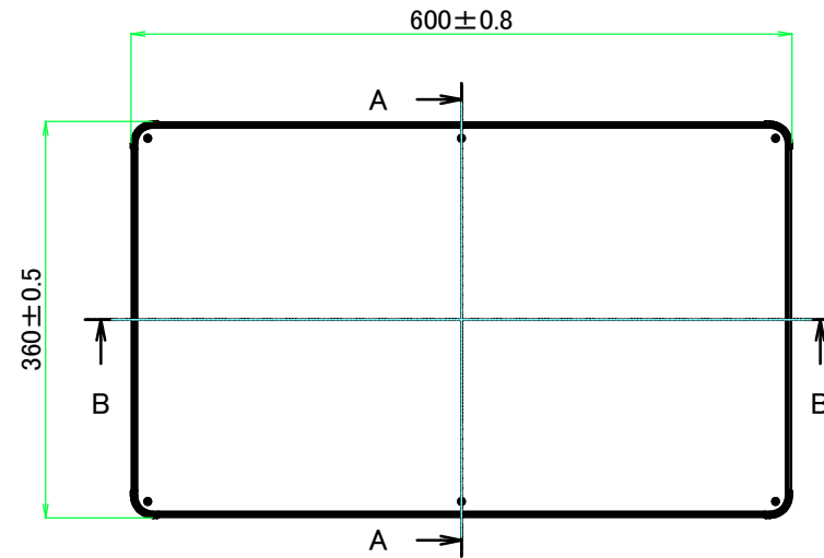
E view
