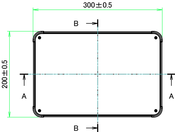
E view
