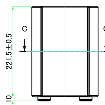
A view
