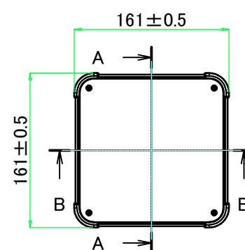
E view
