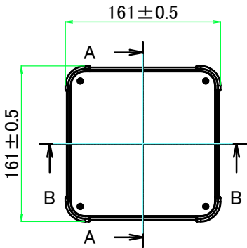
E view
