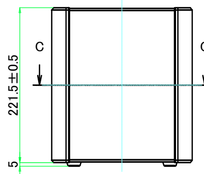
A view
