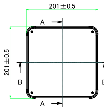
E view
