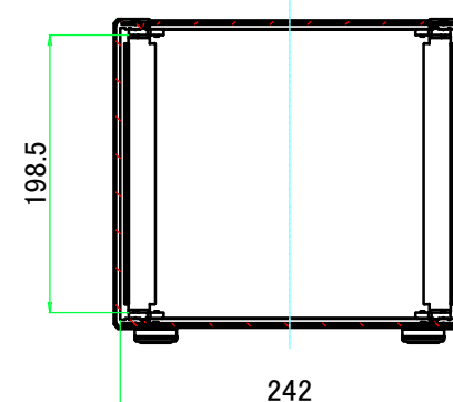
B-B (1:6)
