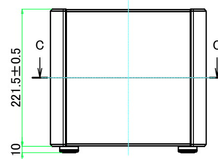
A view
