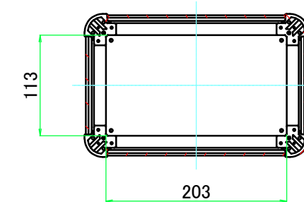
C-C (1:6)
