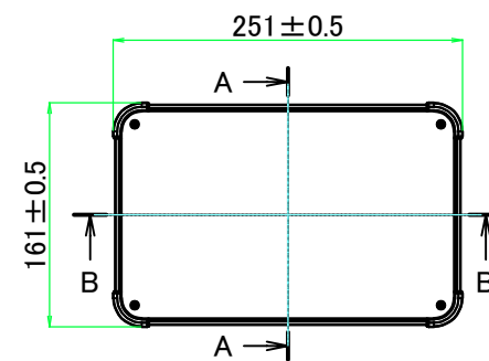
E view
