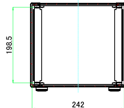
B-B (1:6)
