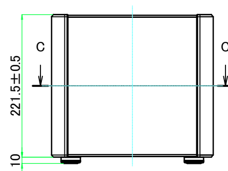
B-B (1:6)
