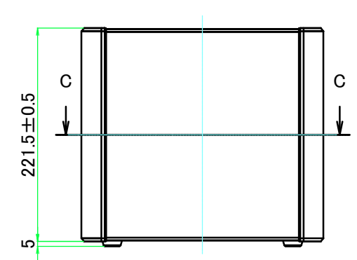
A view
