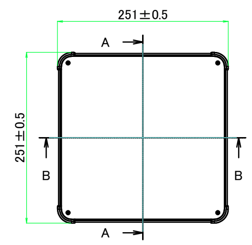
E view
