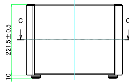
A view
