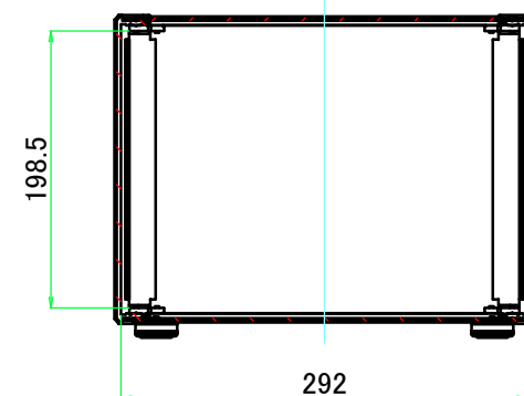
B-B (1:6)
