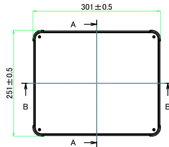
E view
