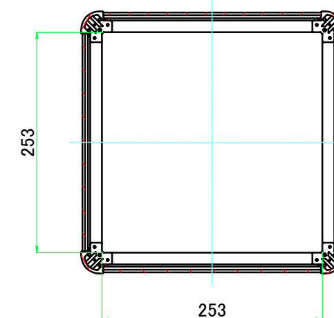
C-C (1:6)
