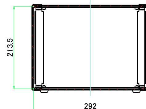
B-B (1:6)
