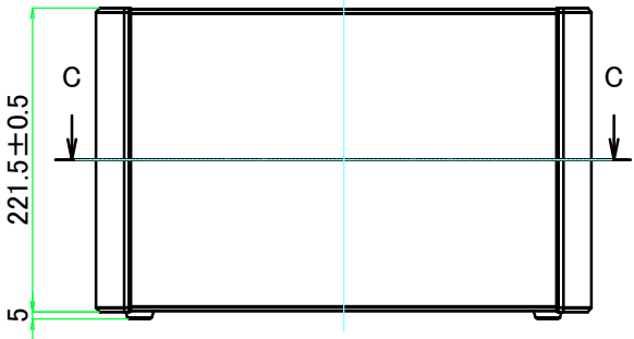
A view
