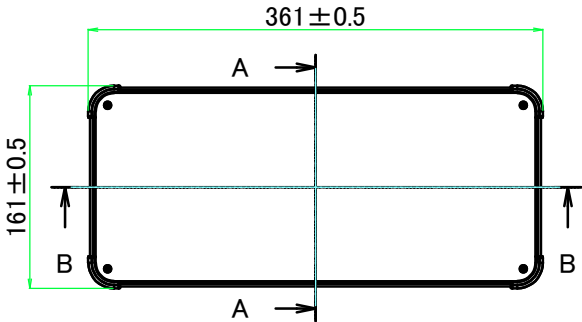
E view
