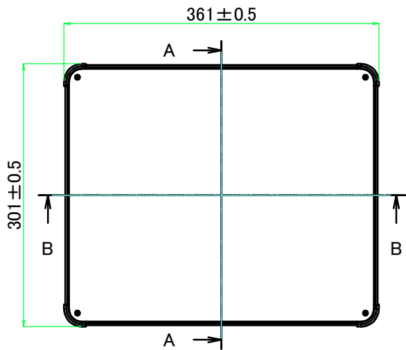
E view
