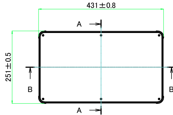
E view
