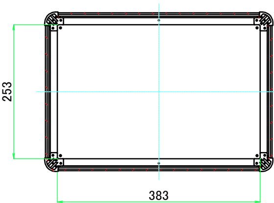
C-C (1:7)
