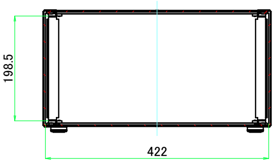
B-B (1:7)
