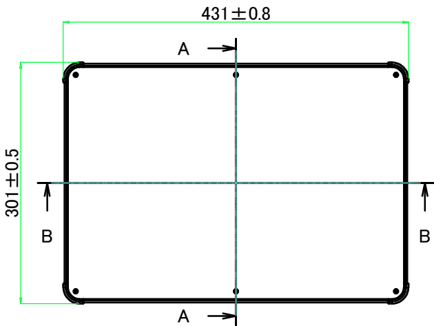
E view
