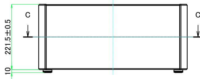
A view
