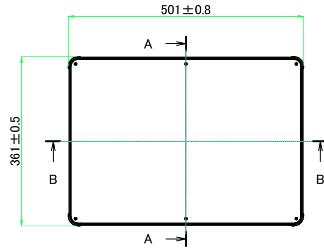
E view
