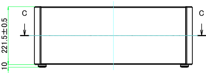
A view
