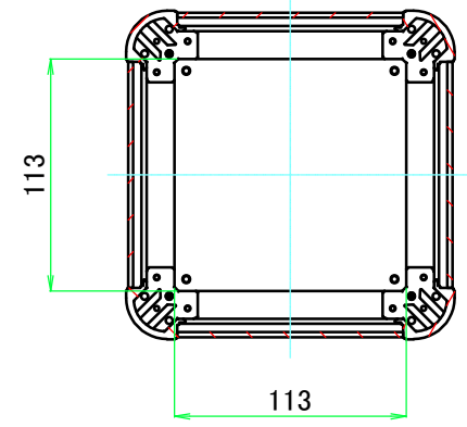
C-C (1:4)
