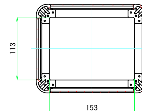
C-C (1:4)
