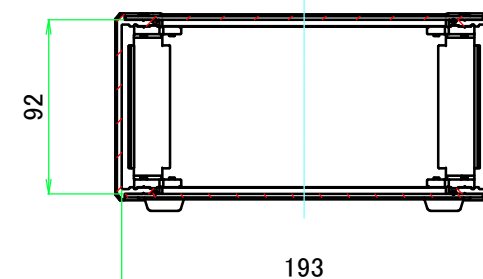
B-B (1:4)
