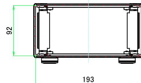
B-B (1:4)
