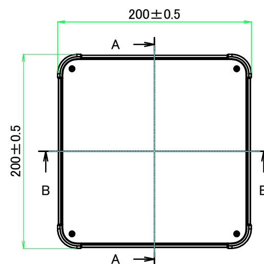
E view
