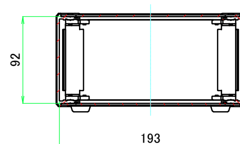
B-B (1:4)
