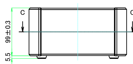
A view
