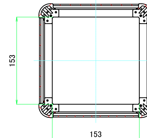
C-C (1:4)
