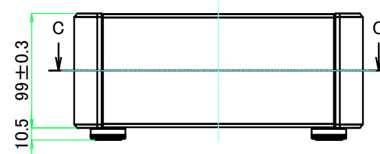
A view
