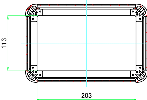
C-C (1:4)
