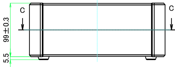
A view
