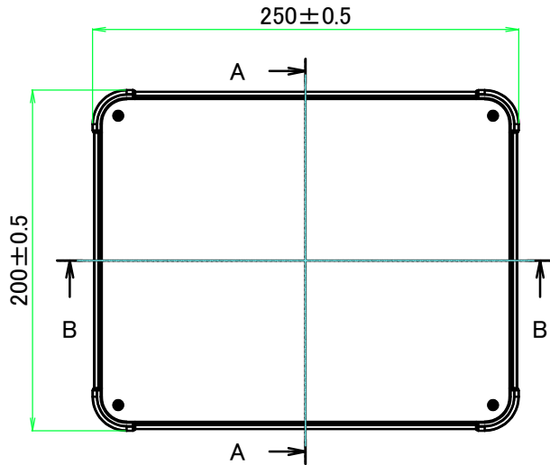
E view
