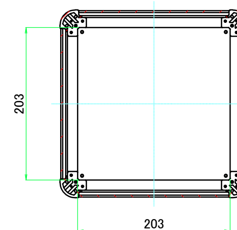
C-C (1:5)
