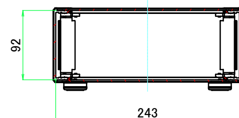
B-B (1:5)
