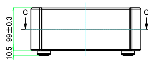
A view
