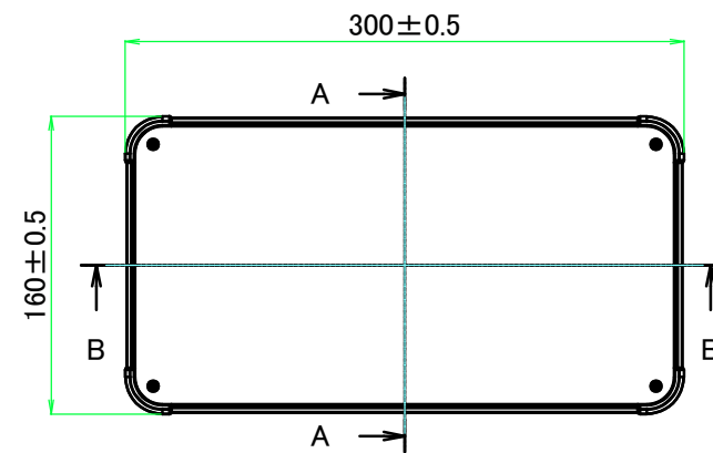
E view
