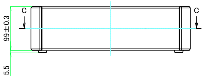
A view
