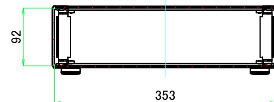
B-B (1:6)
