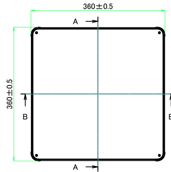
E view
