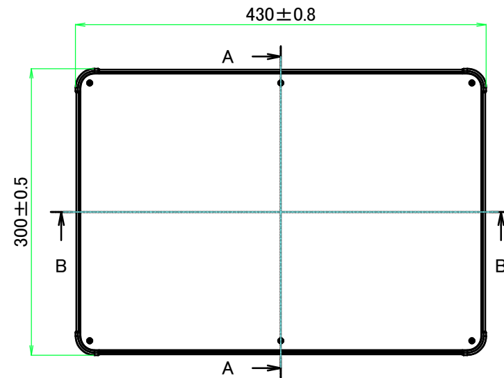
A view
