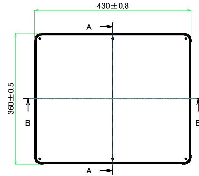
E view
