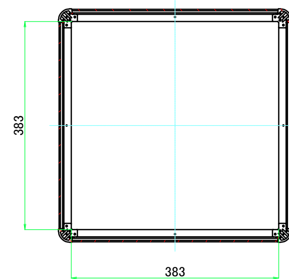
C-C (1:7)
