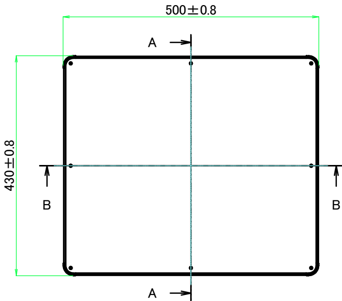
E view
