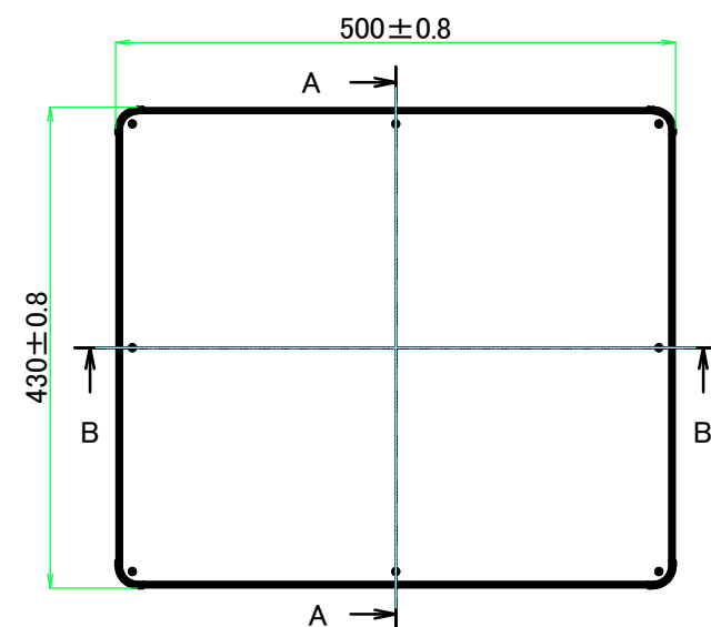
E view
