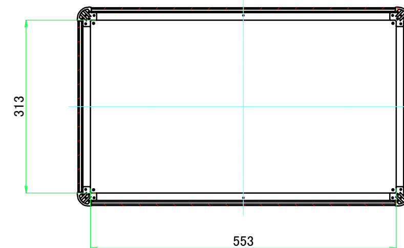
C-C (1:7)
