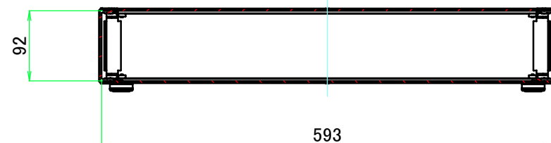
B-B (1:7)
