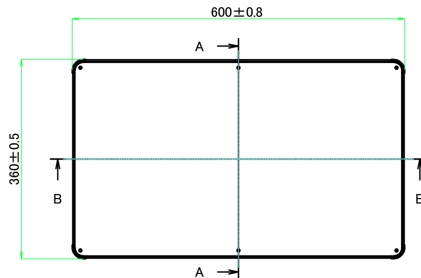
E view
