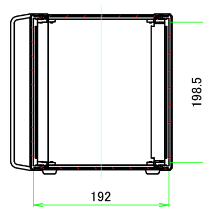
A-A (1:5.5)
