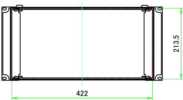
C-C (1:6.5)
