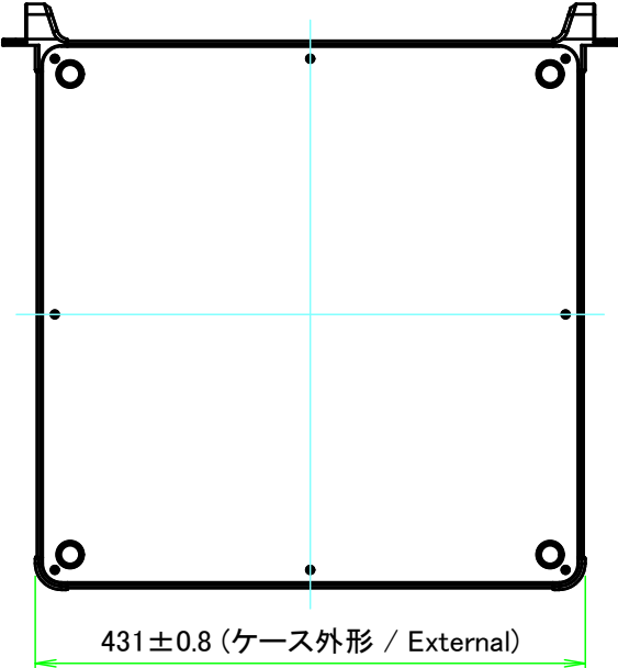
F view
