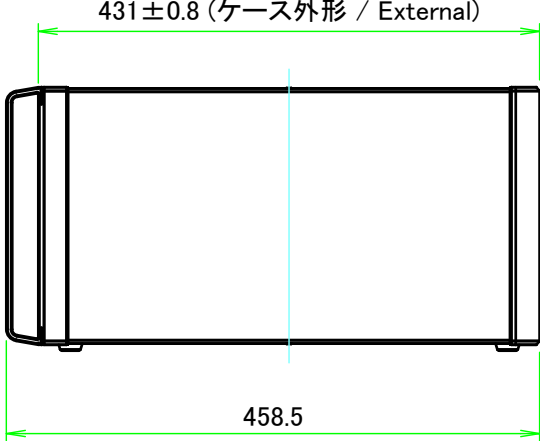
C view
