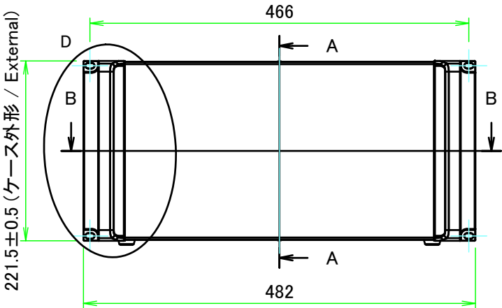
A view
