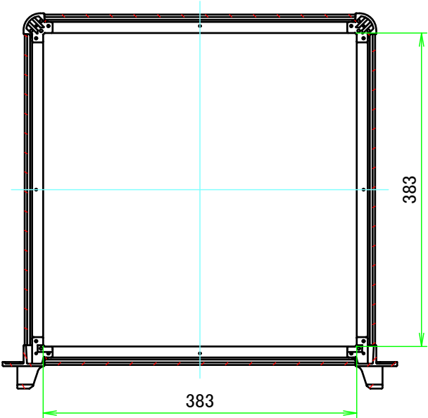
D view
