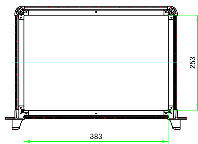
B-B (1:6)
