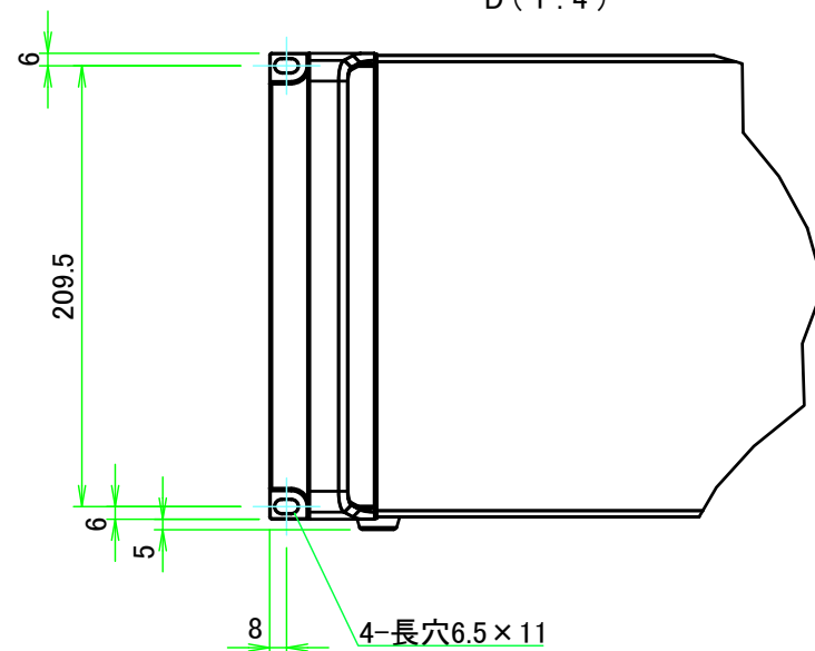
D (1:4)
