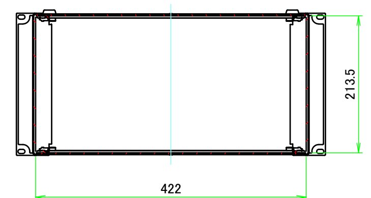
C-C (1:6)
