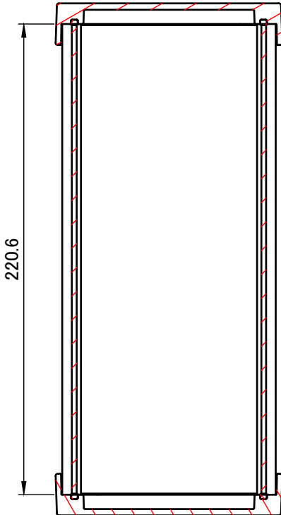
C-C (1:2.5)
