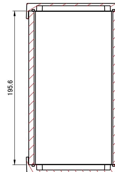
C-C (1:2.5)
