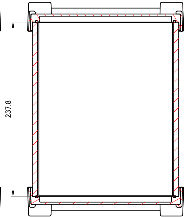
C-C (1:3)
