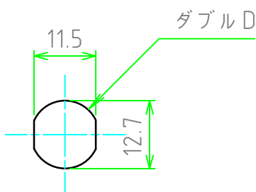
推奨取付穴寸法 Recommended mounting hole dimensions
