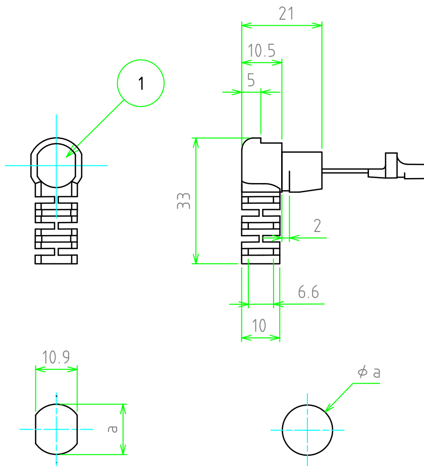
推奨取付穴寸法 Recommended mounting hole dimensions
