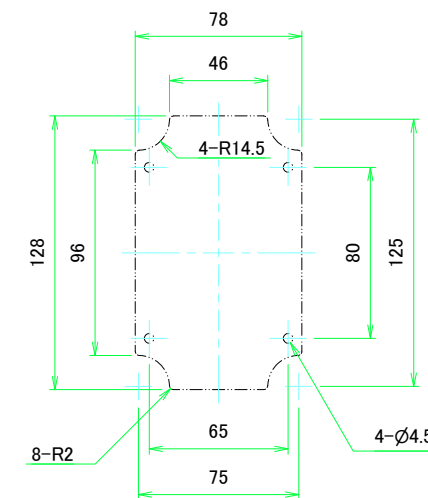
推奨取付ベース形状 Recommended mounting plate dimension
