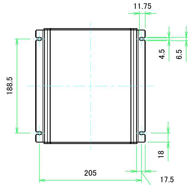
E ( 1 : 1.5 ) detail E
