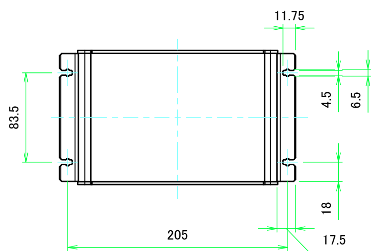
E (1:1) detail E
